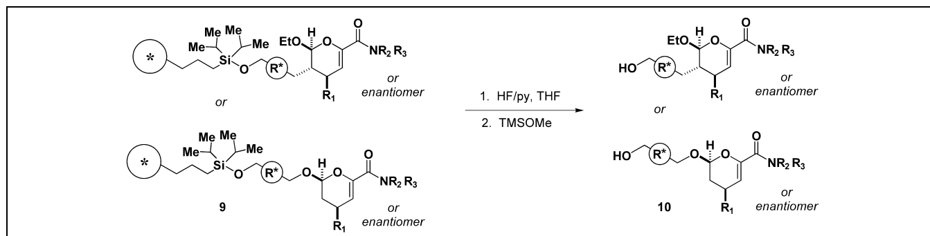
Fig. 7. Cleavage scheme for dihydropyrancarboxamides. Individual beads from separate portions of resin 9 were treated under optimized ‘best practices’ conditions to generate stock solutions of individual members of 10 .
